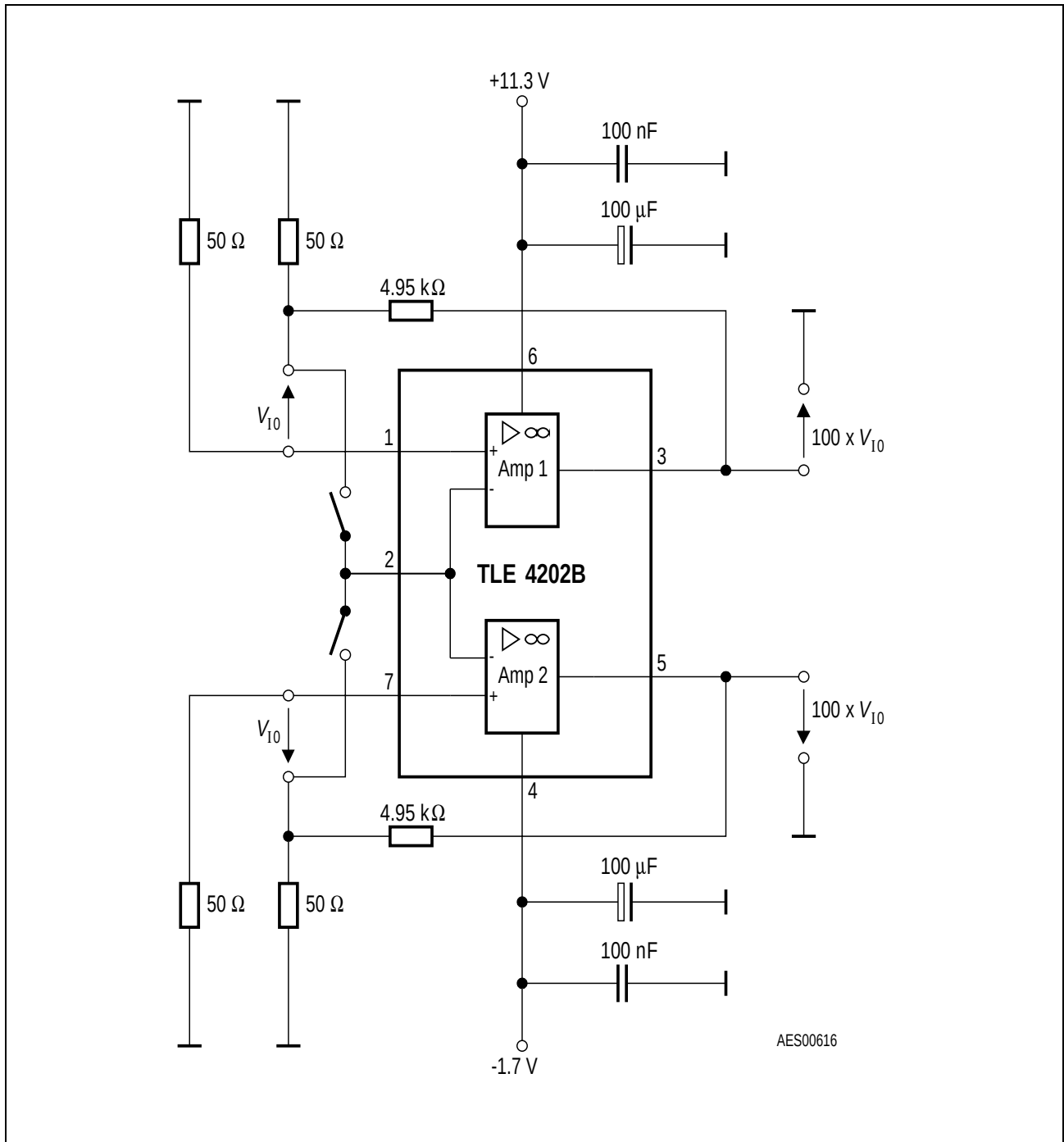
Figure 5 Test Circuit 3
