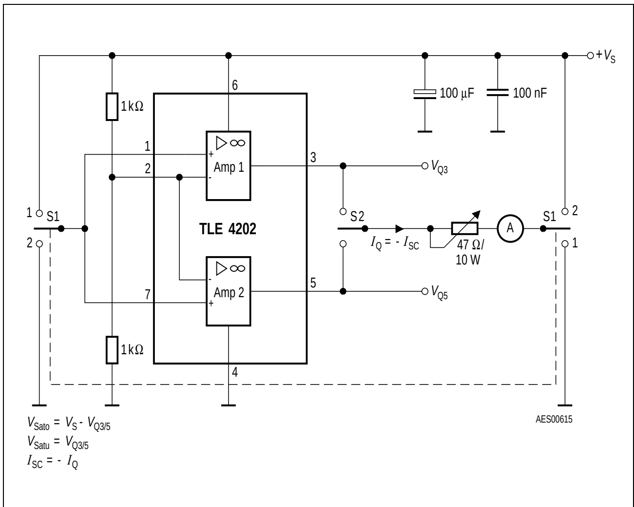
Figure 4 Test Circuit 2
