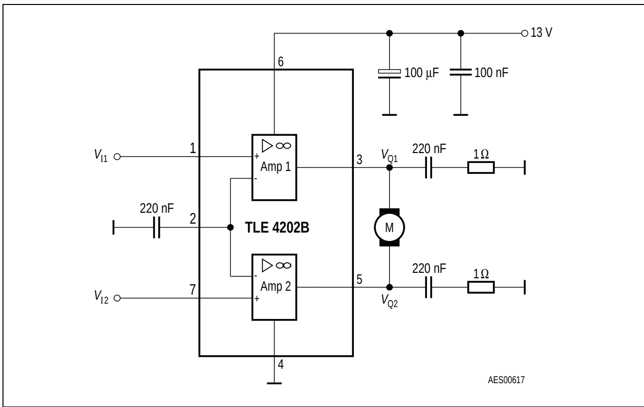
Figure 6 Application Circuit
